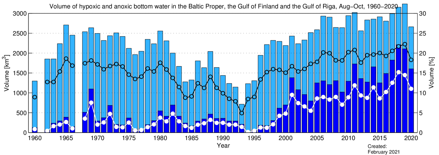
Figure 4. Volume of anoxic and hypoxic deep water in the Baltic Proper, Gulf of Finland and Gulf of Riga. Results from 1961 and 1967 have been removed due to lack of data from the deep basins.
