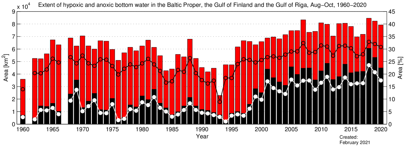
Figure 3. Areal extent of anoxic and hypoxic conditions in the Baltic Proper, Gulf of Finland and Gulf of Riga. Results from 1961 and 1967 have been removed due to lack of data from the deep basins.
