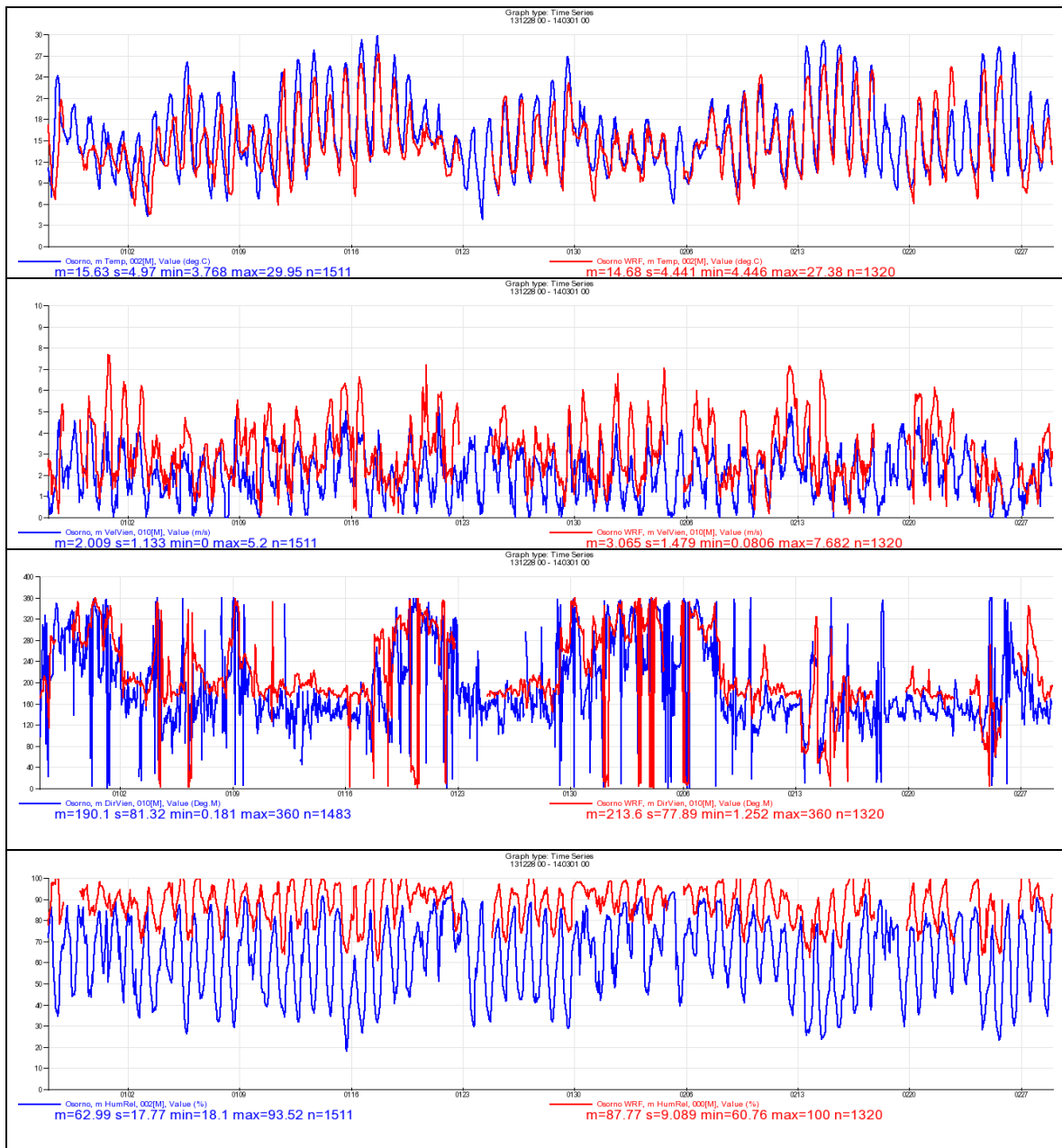
Figure 6.1 Hourly data of WRF simulated (in red) temperature (top), wind speed (top but one), wind direction (bottom but one) and humidity (bottom), as compared to measured meteorology at the El Alba station in Osorno (blue). Period: Dec 28, 2013 – Feb 27, 2014.
