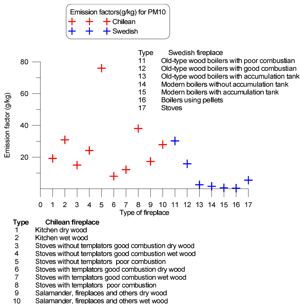
Figure 3.3.5 Comparison between emission factors (g/kg) for PM10 from different fire places used in Chile and Sweden.
